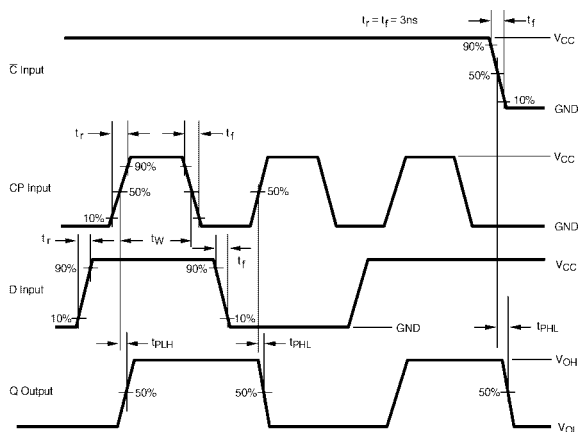
Figure 7. AC Waveforms
