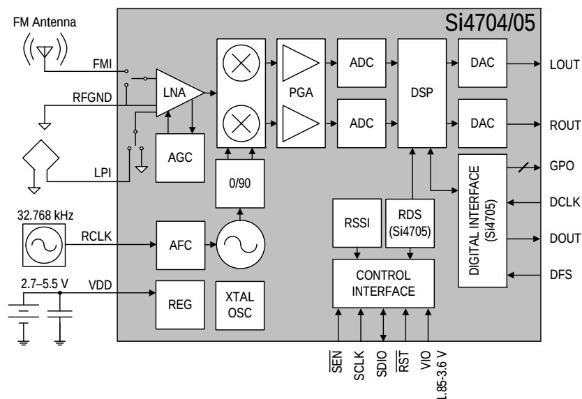
Figure 9. Functional Block Diagram
