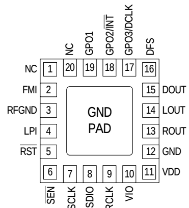
Si4704/05-GM (Top View)
