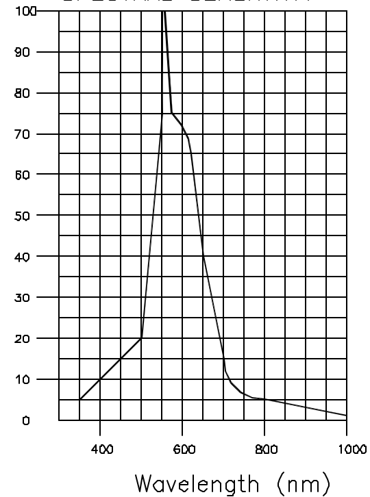
SPECTRAL SENSITIVITY
