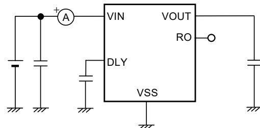
Figure 11 Test Circuit 6
