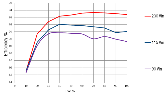
MVAC400-24 Efficiency (including 5V Aux output)
