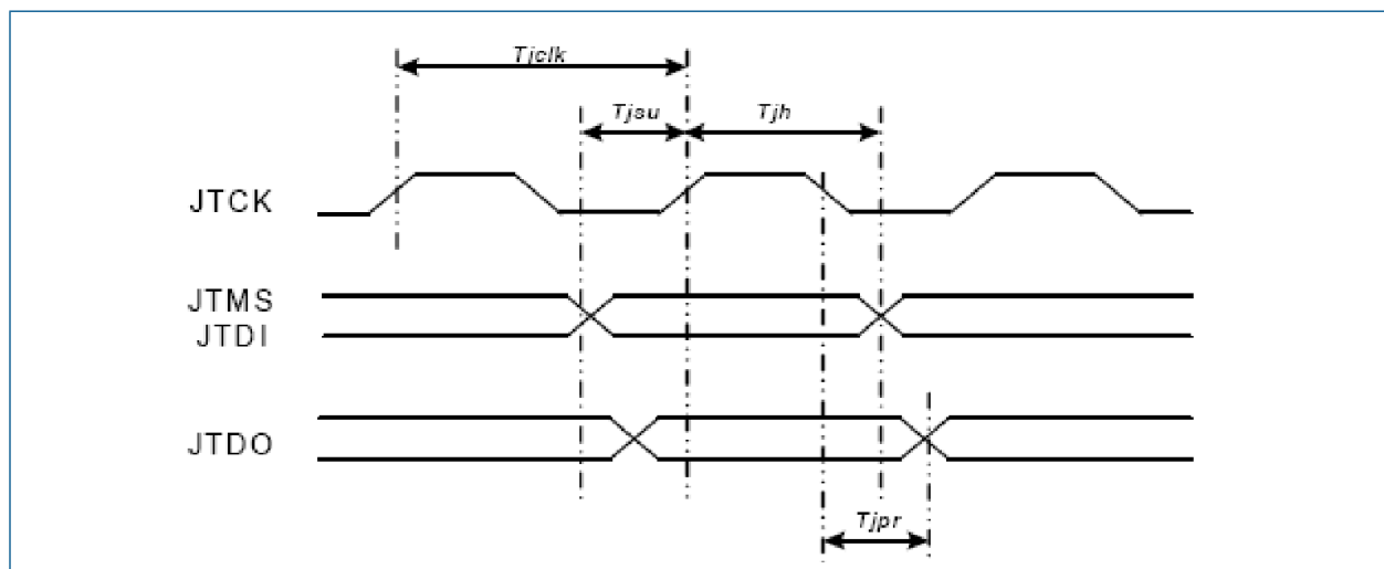
Figure 11-3. JTAG Timing
