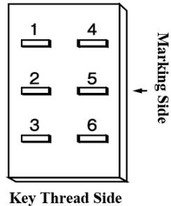
Terminal Diagram
