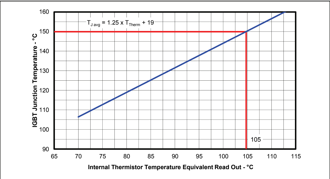
Figure 16 Typical Tj vs Tth correlation, sinusoidal modulation, V_{DC}=300\text{V} , I_{\text{phase}}=5\text{Arms} , f_{sw}=16\text{kHz} , f_{mod}=50\text{Hz} , MI=0.8 , PF=0.6
