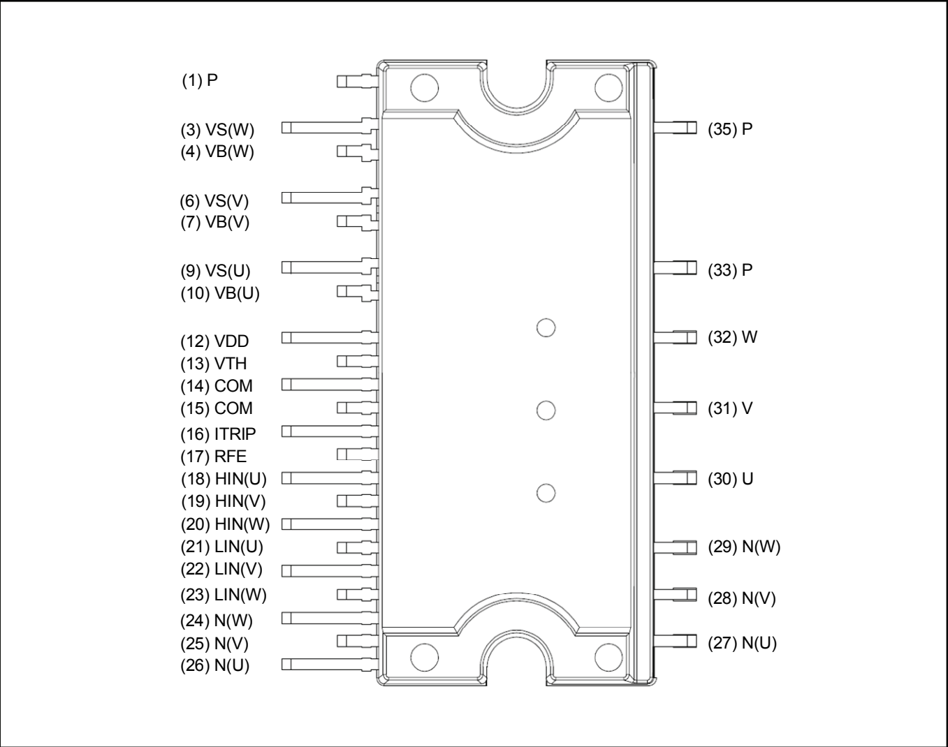
Figure 2 Pin configuration
