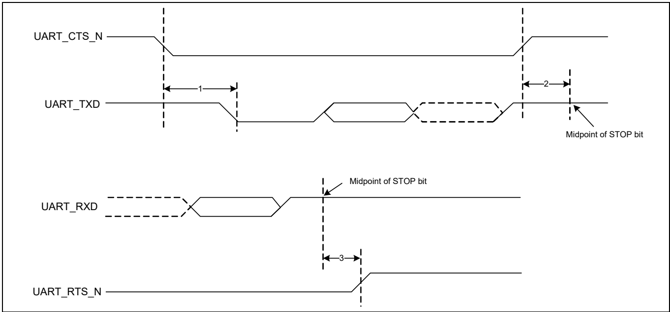
Figure 11 UART timing
