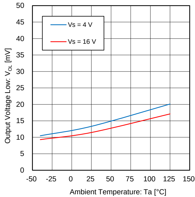
Figure 6. Output Voltage Low vs Ambient Temperature (I L = 1 mA)
