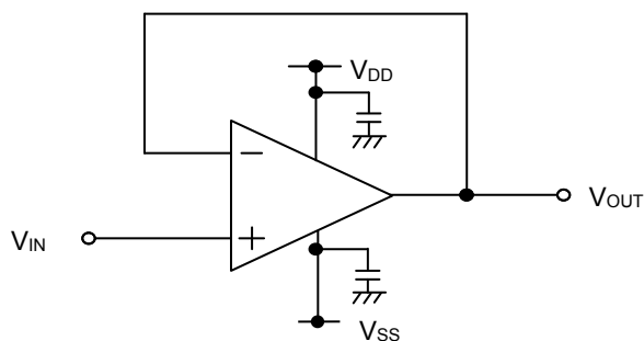
Figure 29. Voltage Follower Circuit
