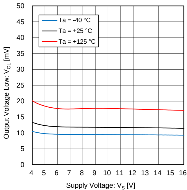
Figure 5. Output Voltage Low vs Supply Voltage (I L = 1 mA)
