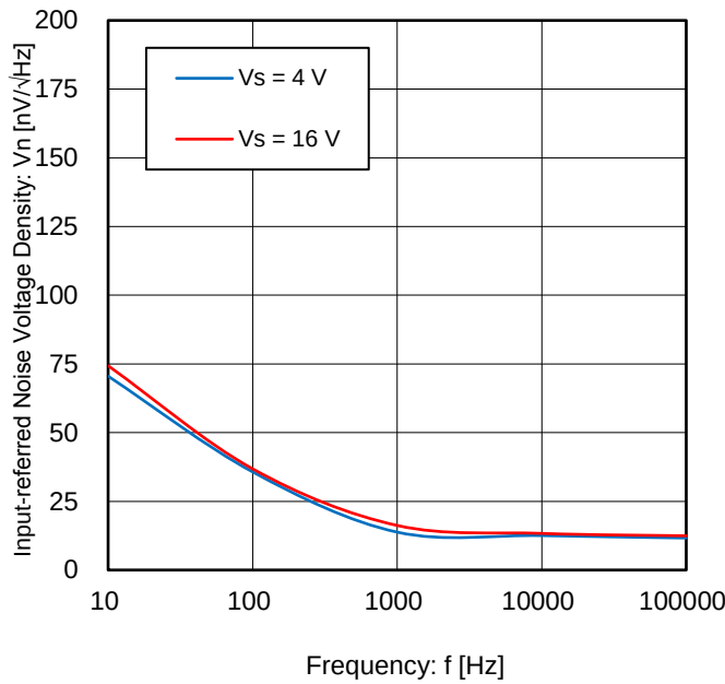
Figure 21. Input-referred Noise Voltage Density vs Frequency
