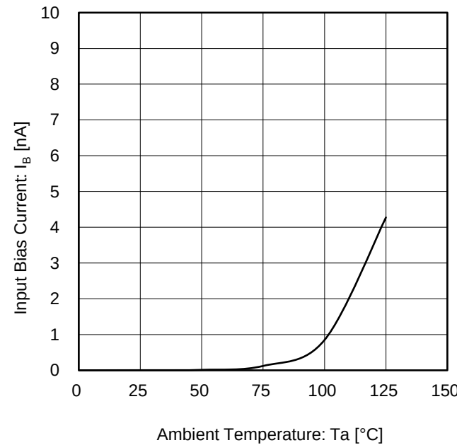
Figure 20. Input Bias Current vs Ambient Temperature
