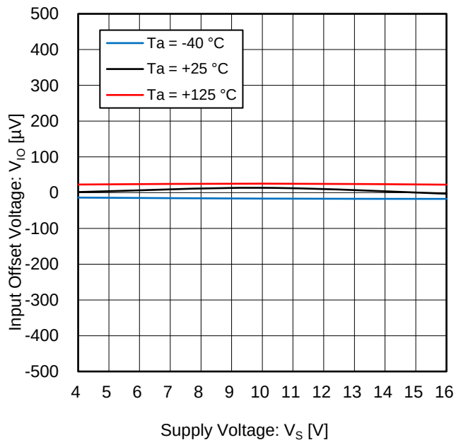
Figure 11. Input Offset Voltage vs Supply Voltage
