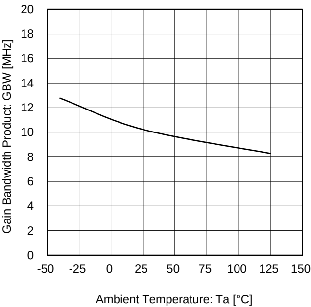
Figure 25. Gain Bandwidth Product: vs Ambient Temperature ( V_S = 10\text{ V} , R_F = 10\text{ k}\Omega , G = 40\text{ dB} )
