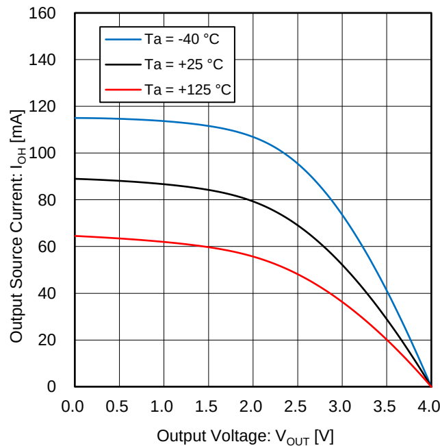
Figure 7. Output Source Current vs Output Voltage (V S = 4 V)
