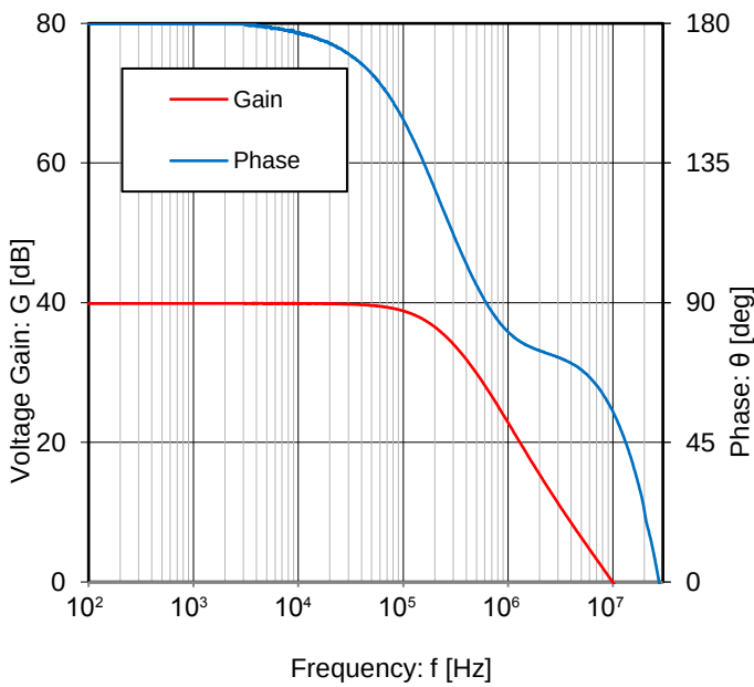
Figure 27. Voltage Gain, Phase vs Frequency ( V_S = 10\text{ V} , R_F = 10\text{ k}\Omega , G = 40\text{ dB} )
