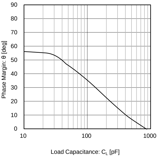
Figure 26. Phase Margin vs Load Capacitance ( V_S = 10\text{ V} , R_F = 10\text{ k}\Omega , G = 40\text{ dB} )
