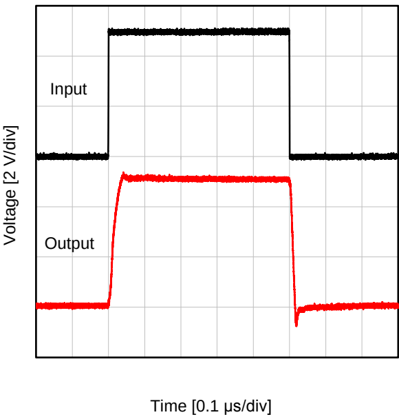
Figure 24. Large-Signal Step Response (V S = 10 V, G = 0 dB, R L = 10 kΩ, C L = 47 pF)
