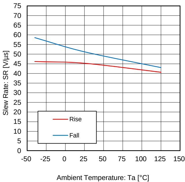
Figure 23. Slew Rate vs Ambient Temperature (V S = 10 V, C L = 50 pF, V IN = 2 Vp-p, G = 0 dB)
