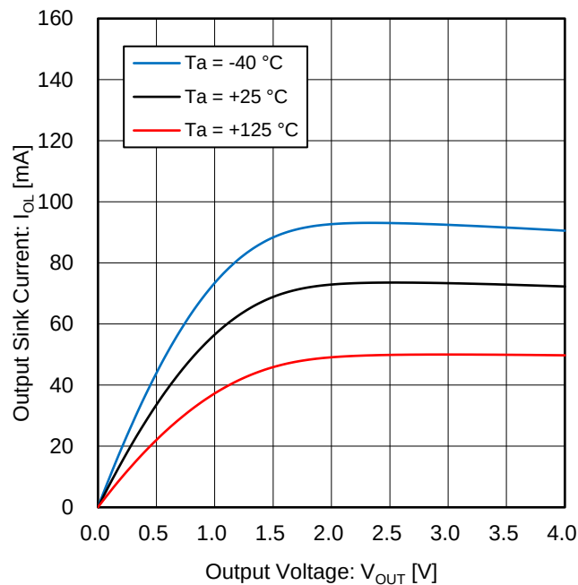
Figure 9. Output Sink Current vs Output Voltage (V S = 4 V)
