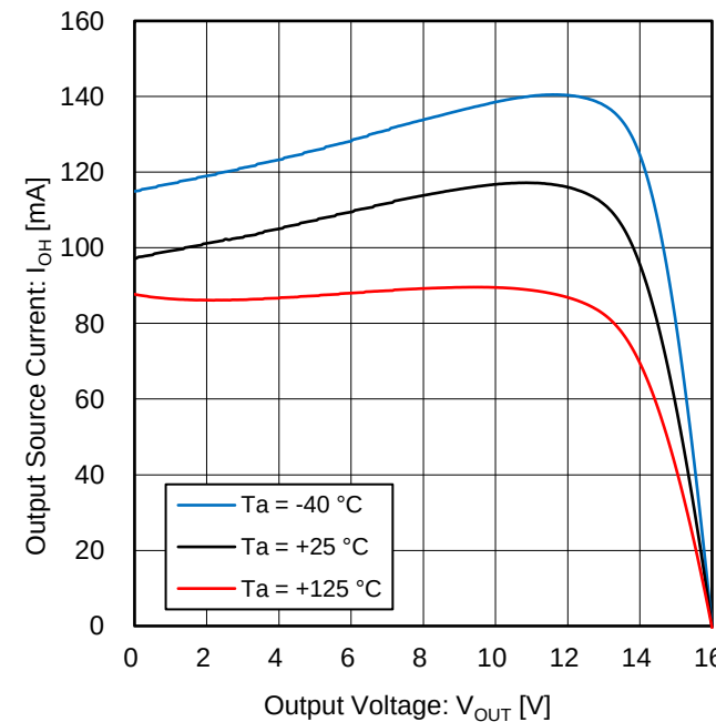
Figure 8. Output Source Current vs Output Voltage (V S = 16 V)
