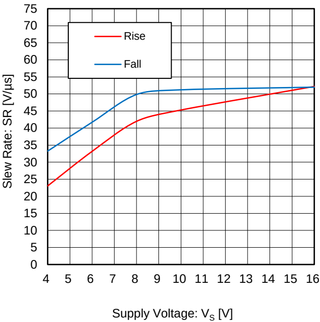
Figure 22. Slew Rate vs Supply Voltage (V S = 10 V, C L = 50 pF, V IN = 2 Vp-p, G = 0 dB)
