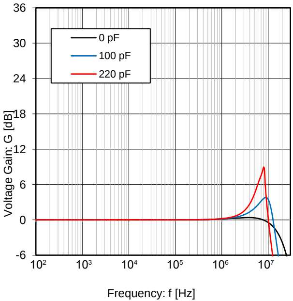
Figure 28. Voltage Gain vs Frequency ( V_S = 10\text{ V} , G = 0\text{ dB} , V_{IN} = 180\text{ mVp-p} )
