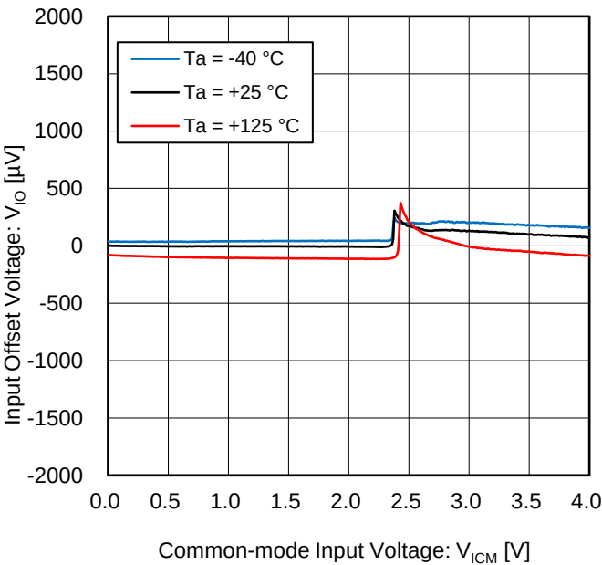
Figure 13. Input Offset Voltage vs Common-mode Input Voltage ( V_S = 4\text{ V} )
