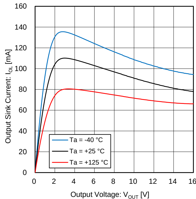
Figure 10. Output Sink Current vs Output Voltage (V S = 16 V)
