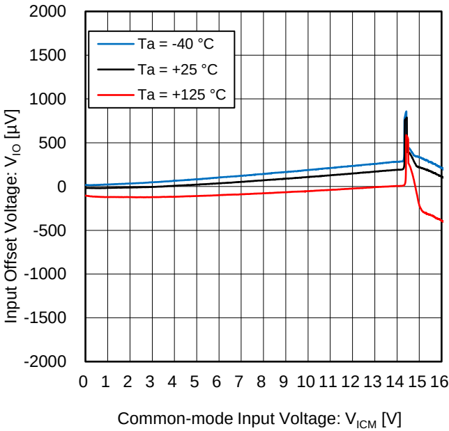
Figure 14. Input Offset Voltage vs Common-mode Input Voltage ( V_S = 16\text{ V} )
