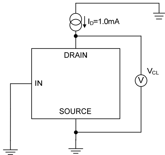
Figure 6. Output Clamp Voltage Measuring Circuit
