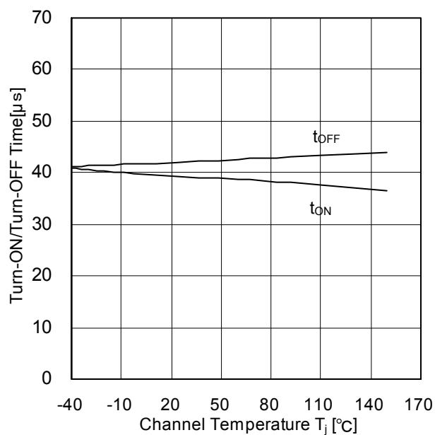
Figure 14. Turn-ON / Turn-OFF Time vs. Junction Temperature
