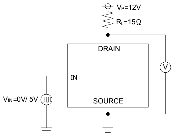
Figure 8. t ON • t OFF Measuring Circuit
