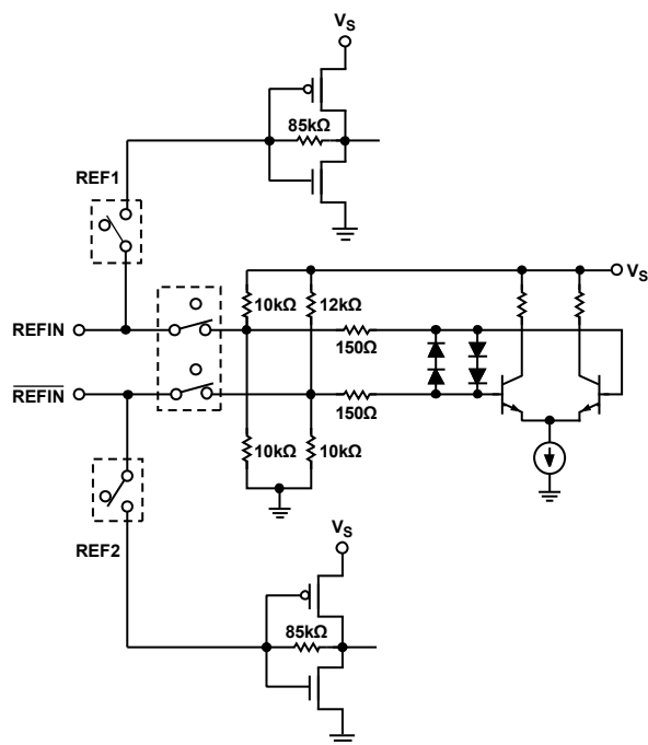
Figure 34. REF1N Equivalent Circuit
