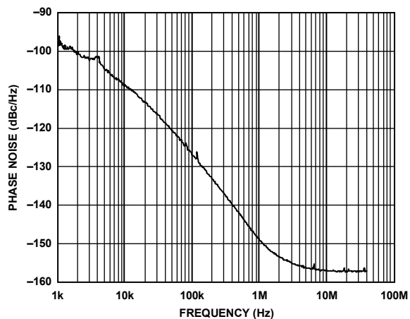
Figure 24. Phase Noise (Absolute) Clock Cleanup; Internal VCO at 1.556 GHz; PFD = 19.44 MHz; LBW = 12.8 kHz; LVPECL Output = 155.52 MHz
