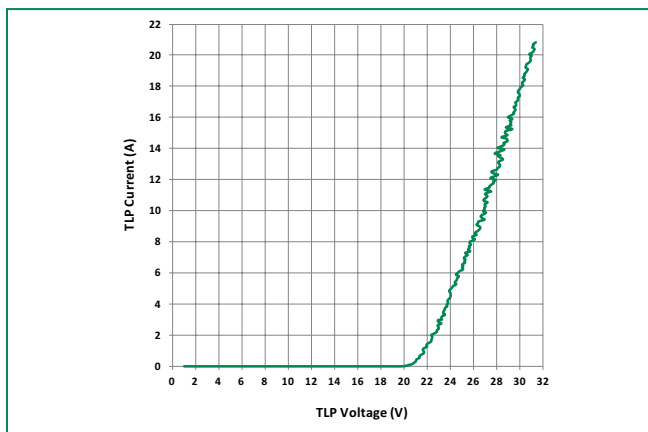
AQ15C Transmission Line Pulsing(TLP) Plot
