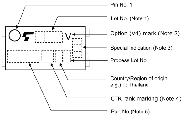
Fig. 15.3 Marking Example
