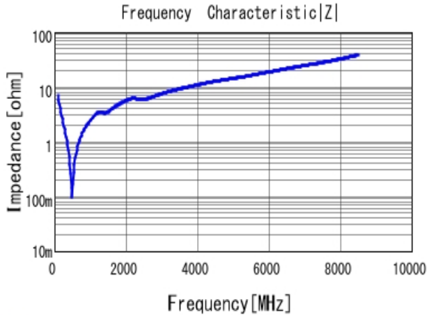
■ GRM2165C2A221JA01 |Z| DC0V, 25degC
