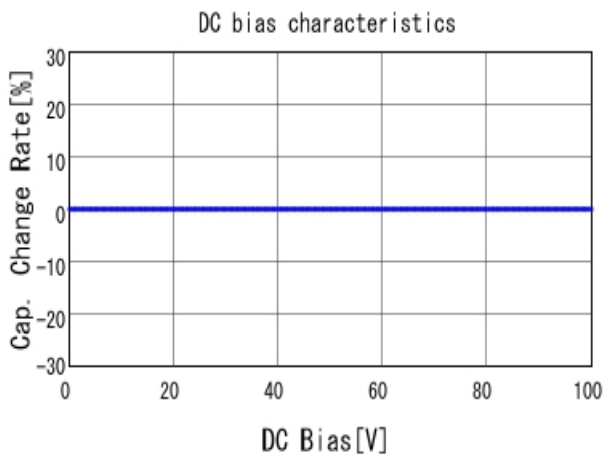
■ GRM2165C2A221JA01 C-DC bias capchange, 25.0degC, AC1V
