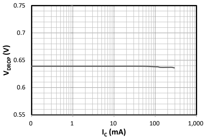
Figure 3. V_{DROP} vs I_C
