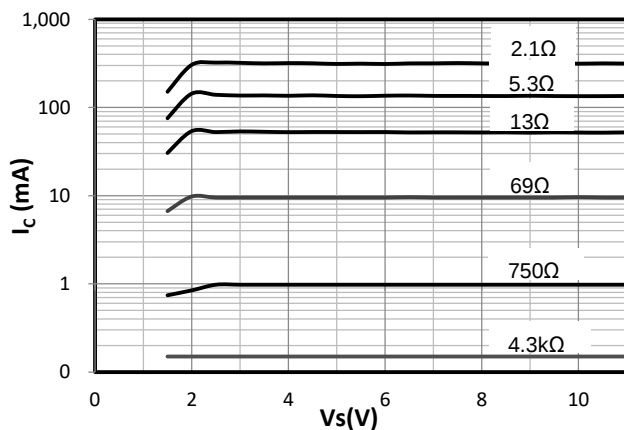
Figure 5. I_C vs. V_S (Parameter R_{EXT}=(\Omega) )
