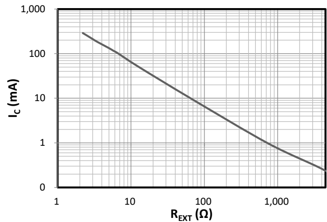
Figure 4. V_{EN} vs I_{OUT} ( R_{EXT}=open )
