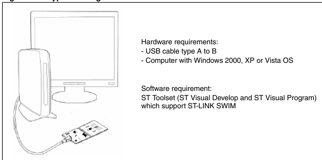
Figure 6. Typical configuration
