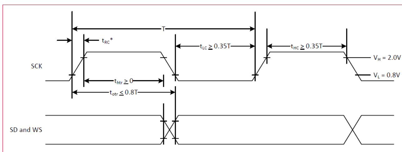
Figure 13: I 2 S Transmitter Timing
