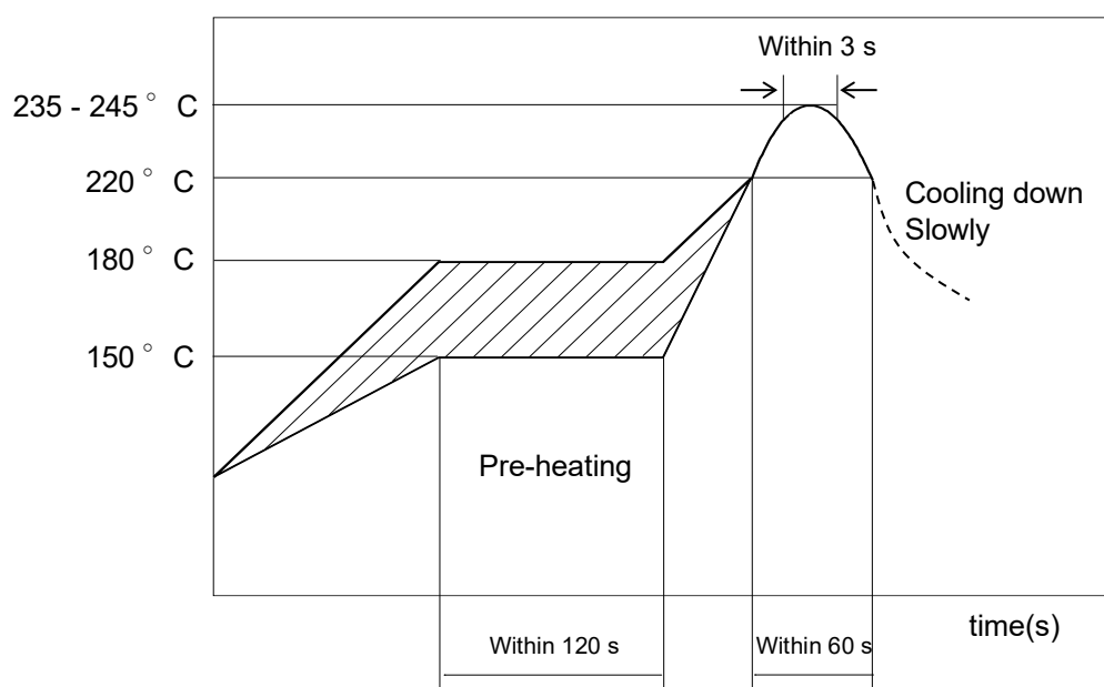
Figure 31: Reflow Soldering Standard Conditions (Example)
