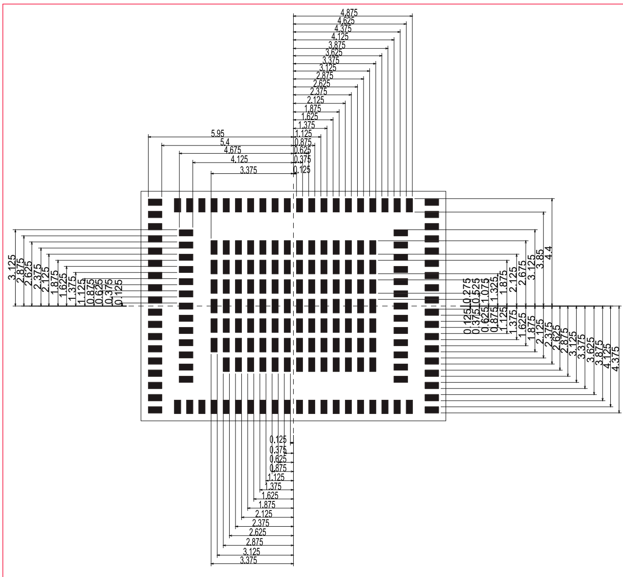
Figure 24: Land Pattern (Top View)
