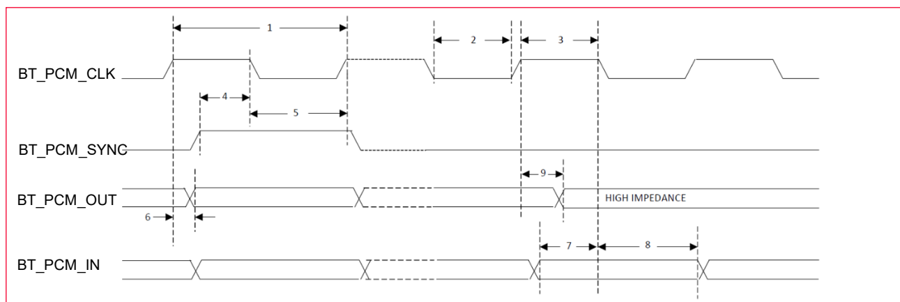
Figure 10: Short Frame Sync, Slave Mode
