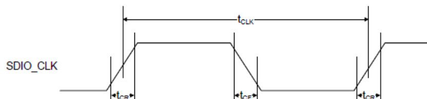
Figure 22: SDIO Clock Timing (DDR50 Mode)
