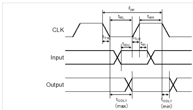
Figure 15: SDIO Default Mode Timing
