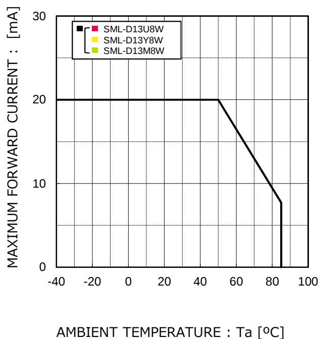
Fig.4 Derating
