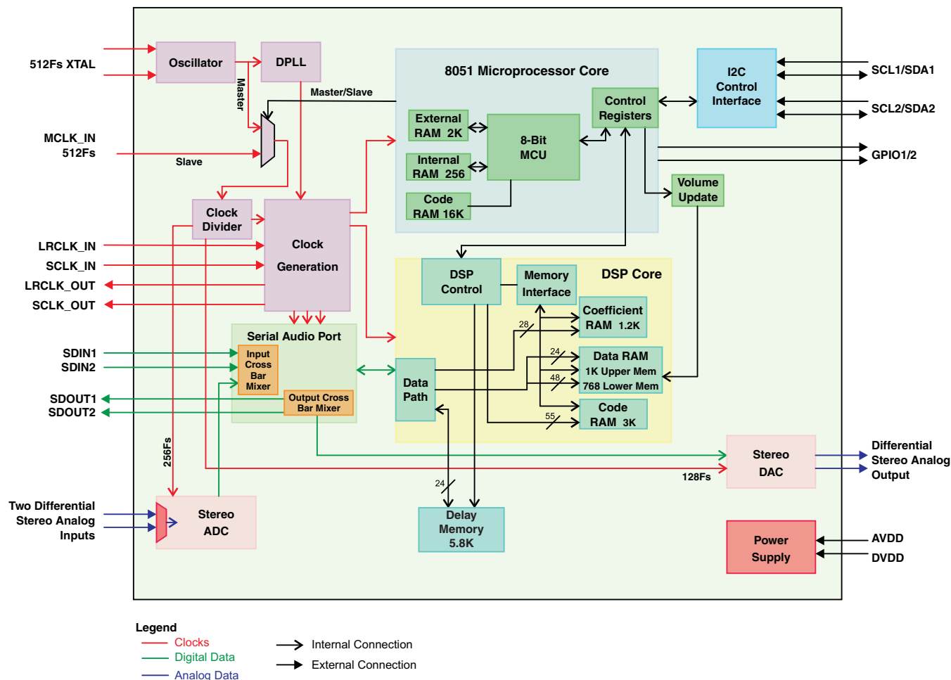
Figure 1-1. Expanded Functional Block Diagram
