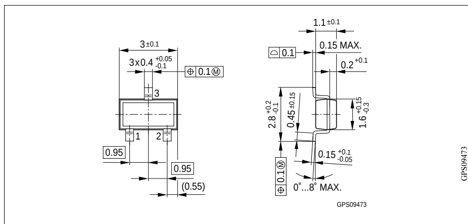
Figure 6 SC59
