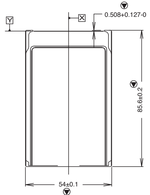
Top Cover
