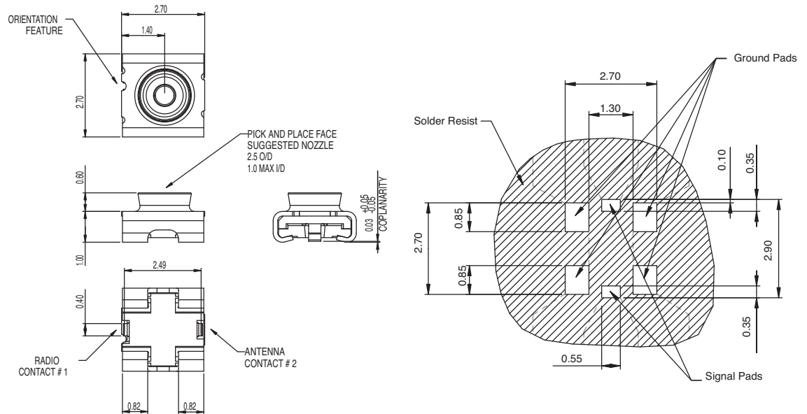
120220-0180 Cradle Interface
