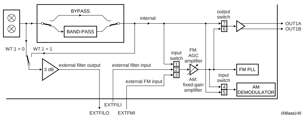
Fig 9. Signal path for intercarrier (2nd SIF) processing
