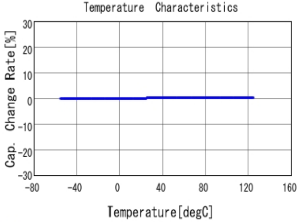
■ GRM1885C1H1R8CA01 C-Temp. capchange, DCOV, AC1Vrms
