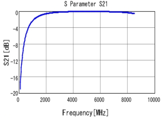
■ GRM1885C1H1R8CA01 S21 DCOV, 25degC
