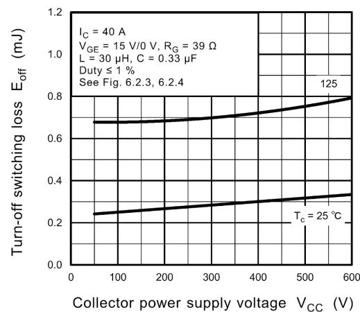
Fig. 8.14 E_{off} - V_{CC}
