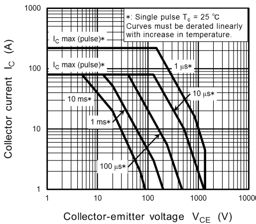
Fig. 8.10 Safe Operating Area (Guaranteed Maximum)
