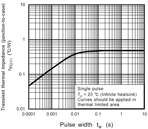
Fig. 8.9 r_{th(j-c)} - t_w (Guaranteed Maximum)
