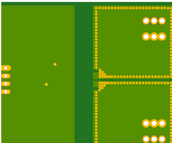
Figure 44: Recommended PCB Layout (Bottom Layer) for the 20 A to 65 A variants of the CT418
