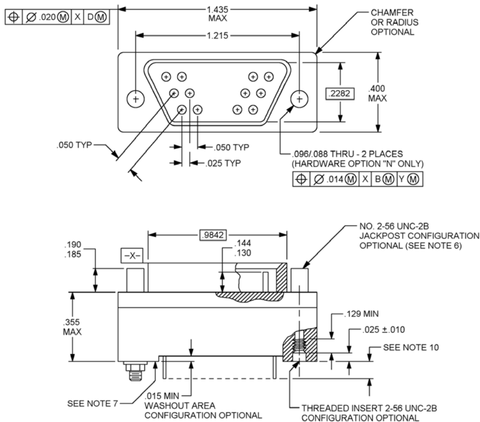
FIGURE 1. Connector receptacle.
