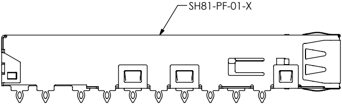
FIG 4 QSFP-C-PF-01-F SHOWN (SAME AS FIG 1, EXCEPT AS SHOWN) (SEE NOTE 6)
