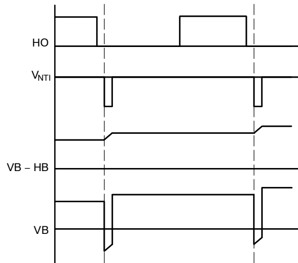
Figure 30. Timing Diagram
