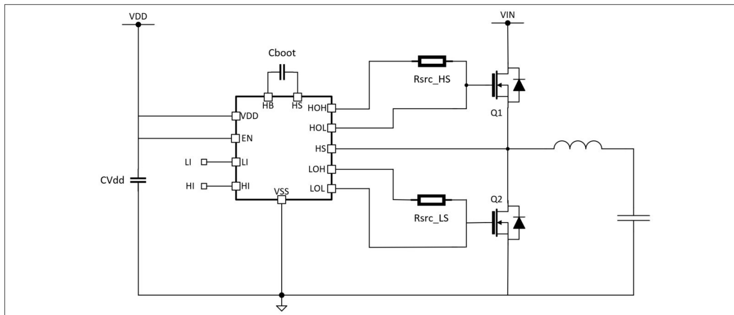
Figure 26 Typical application
