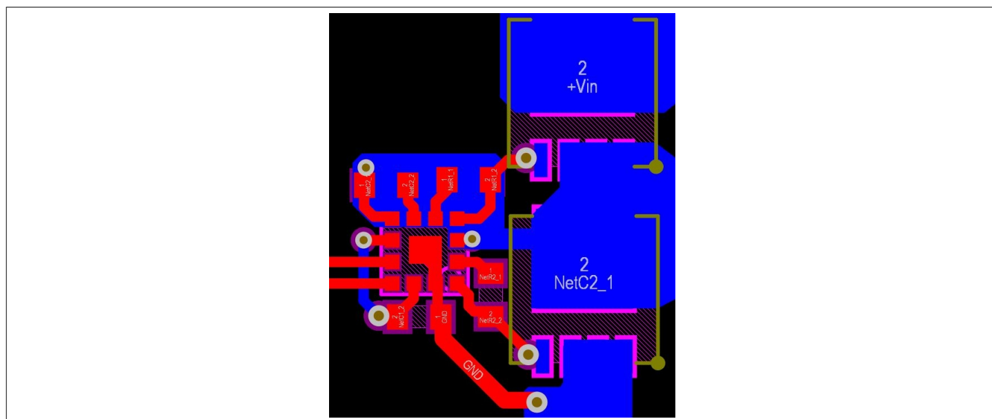
Figure 31 2EDL50X3U2D Layout example in a half-bridge configuration
