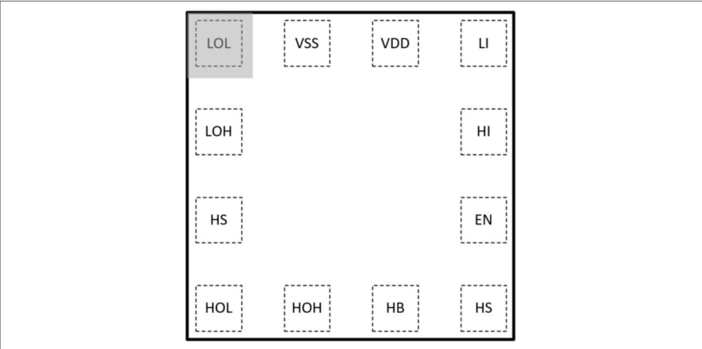
Figure 1 Top view
