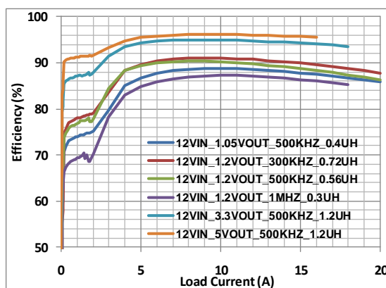
Figure 11. Efficiency vs. Load Current with V_{IN}=12\text{ V}
