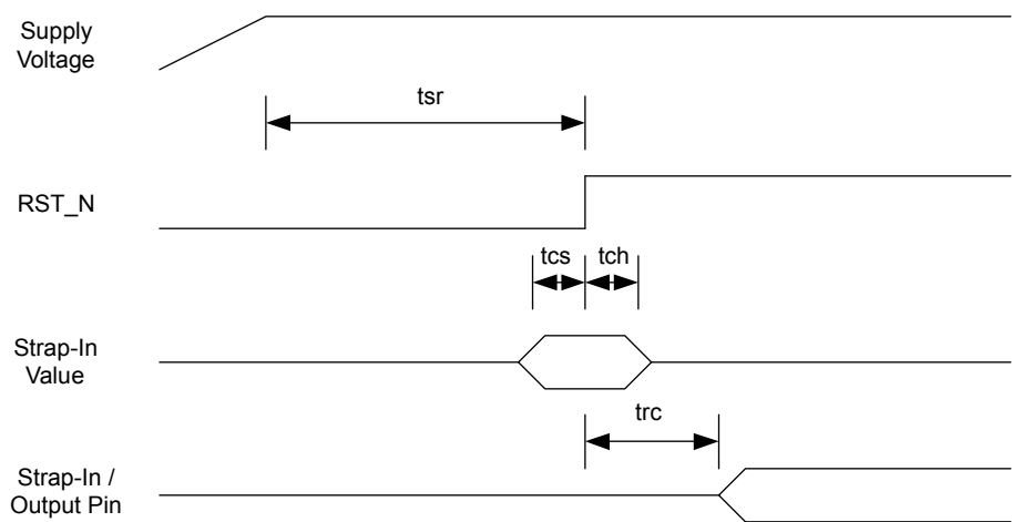
Figure 15. Reset Timing
