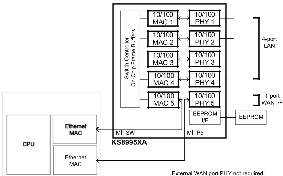
Figure 1. Broadband Gateway
