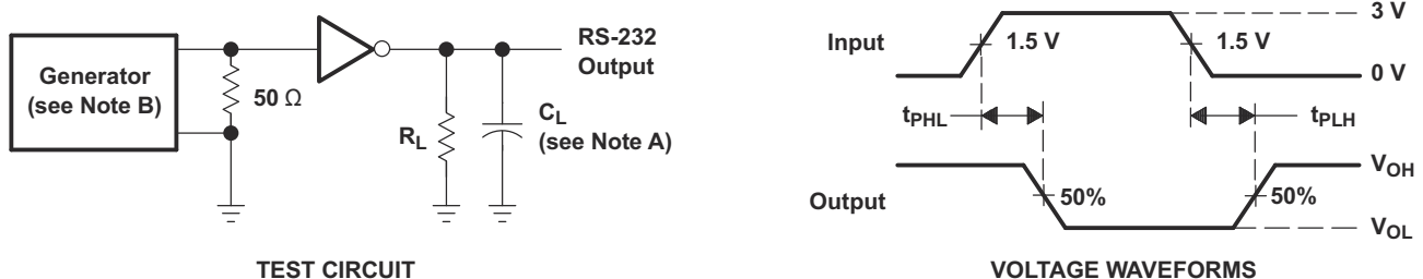
Figure 7-1. Driver Slew Rate
