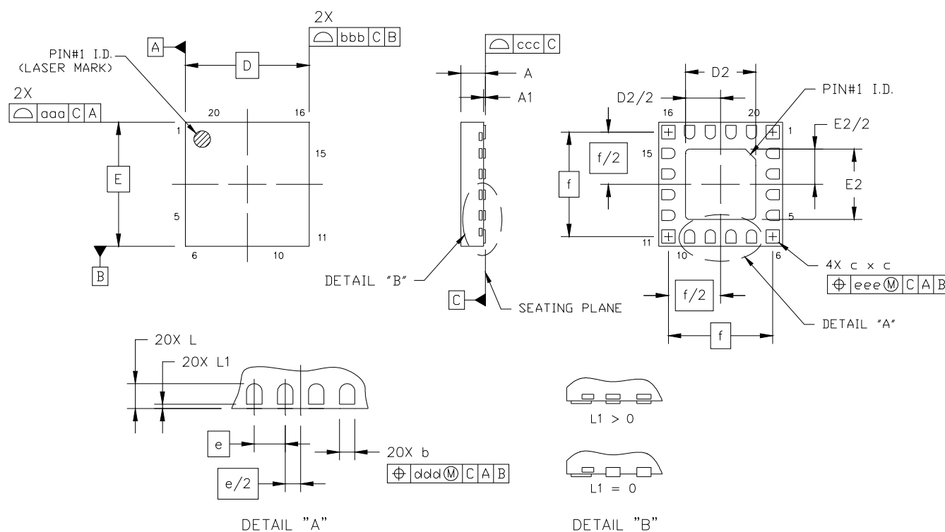
Figure 16. 20-Pin Quad Flat No-Lead (QFN)
