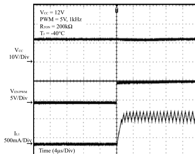
Figure 21 PWM On
