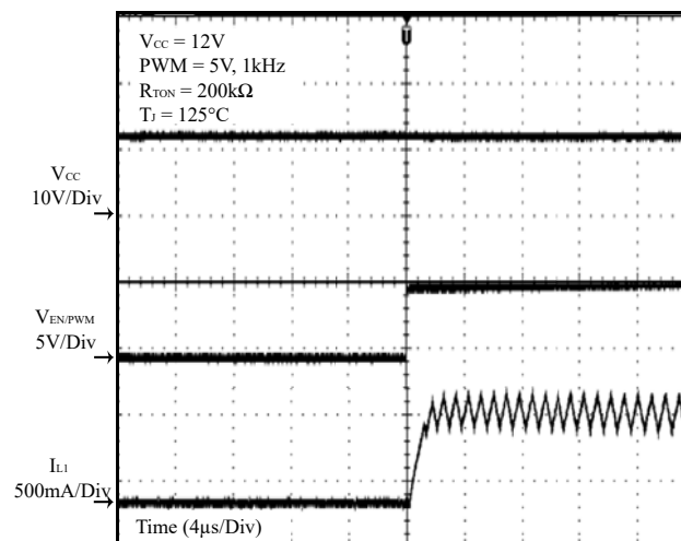
Figure 25 PWM On
