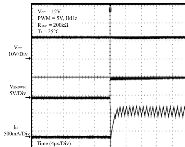
Figure 23 PWM On
