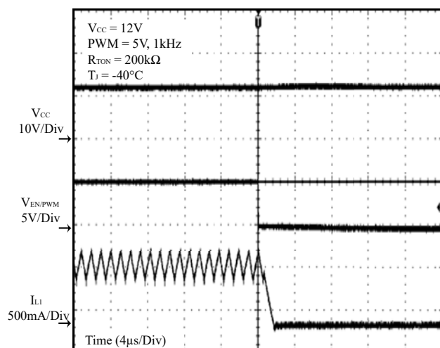
Figure 20 PWM Off
