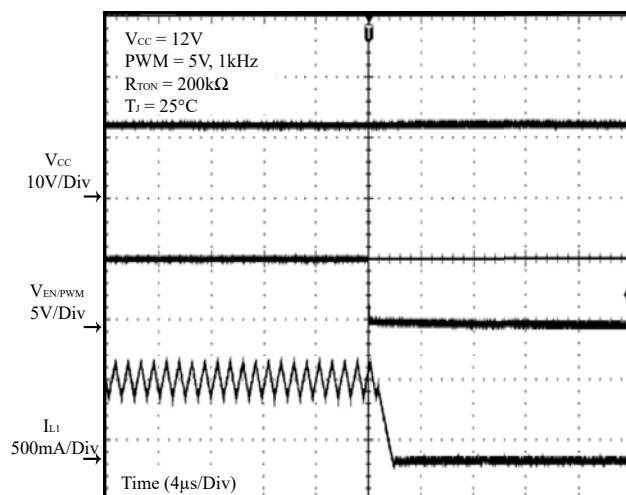
Figure 22 PWM Off
