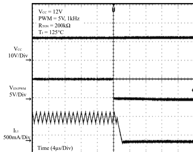
Figure 24 PWM Off
