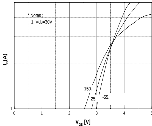
Fig.5 Transfer Characteristics
