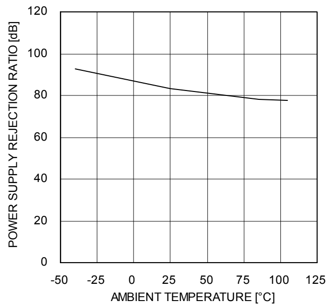
Figure 67. Power Supply Rejection Ratio vs Ambient Temperature
