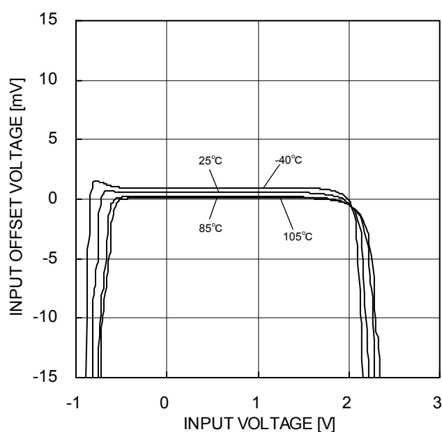
Figure 62. Input Offset Voltage vs Common Mode Input Voltage (VDD=3V)
