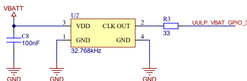
Figure 8.12. 32.768 kHz Clock Oscillator
