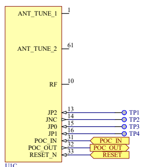
Figure 8.9. RF, Debug, and Reset Connection
