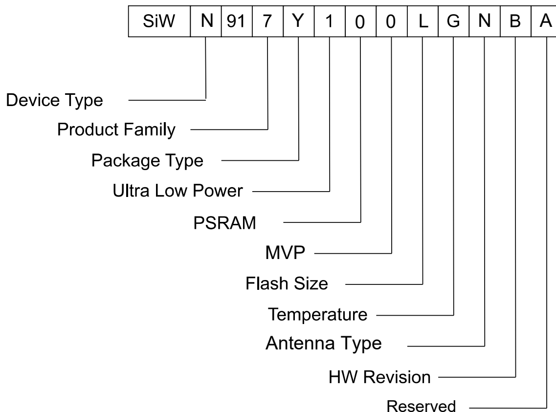
Figure 2.1. Ordering Guide
