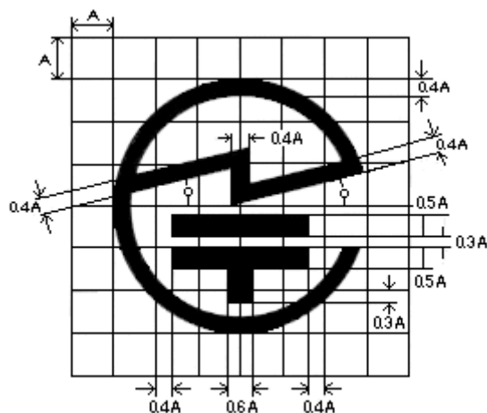
Figure 12.2. Detail of "Giteki" Technical Conformity Mark
