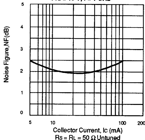
NE46100, NE46134 NOISE FIGURE vs. COLLECTOR CURRENT V_{CE} = 10\text{ V} , f = 1\text{ GHz}
