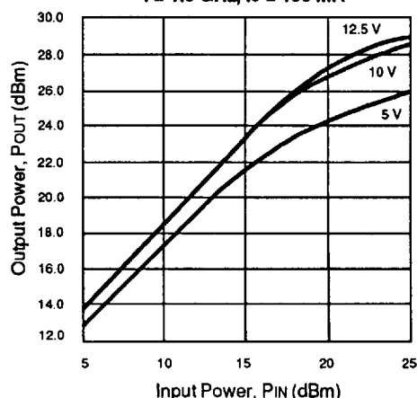
NE46134 TYPICAL OUTPUT POWER vs. INPUT POWER f = 1.0 \text{ GHz} , I_c = 100 \text{ mA}
