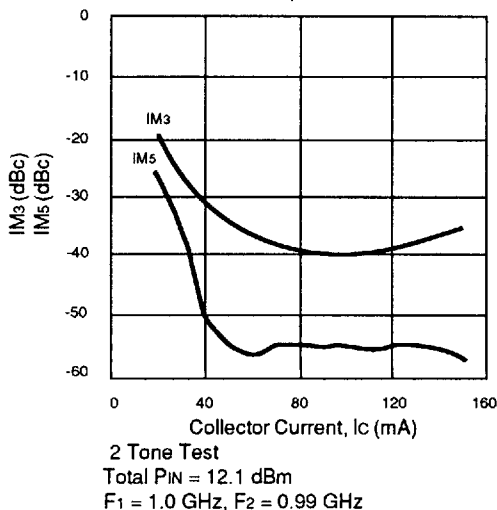
NE46100, NE46134 INTERMODULATION DISTORTION vs. COLLECTOR CURRENT f = 1.0\text{ GHz} , V_{CE} = 10\text{ V}
