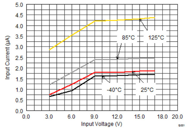
Figure 2. Shutdown Current
