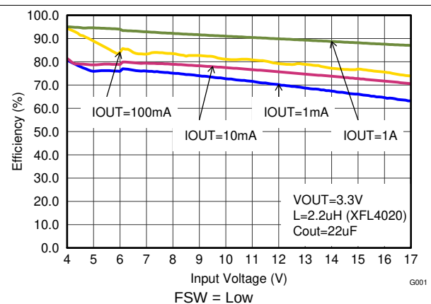
Figure 17. Efficiency versus Input Voltage
