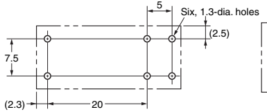
PCB Mounting Holes (Bottom View)
