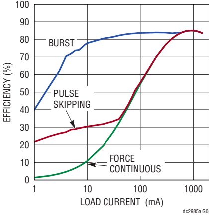
BUCK4 1.81V OUT Efficiency
