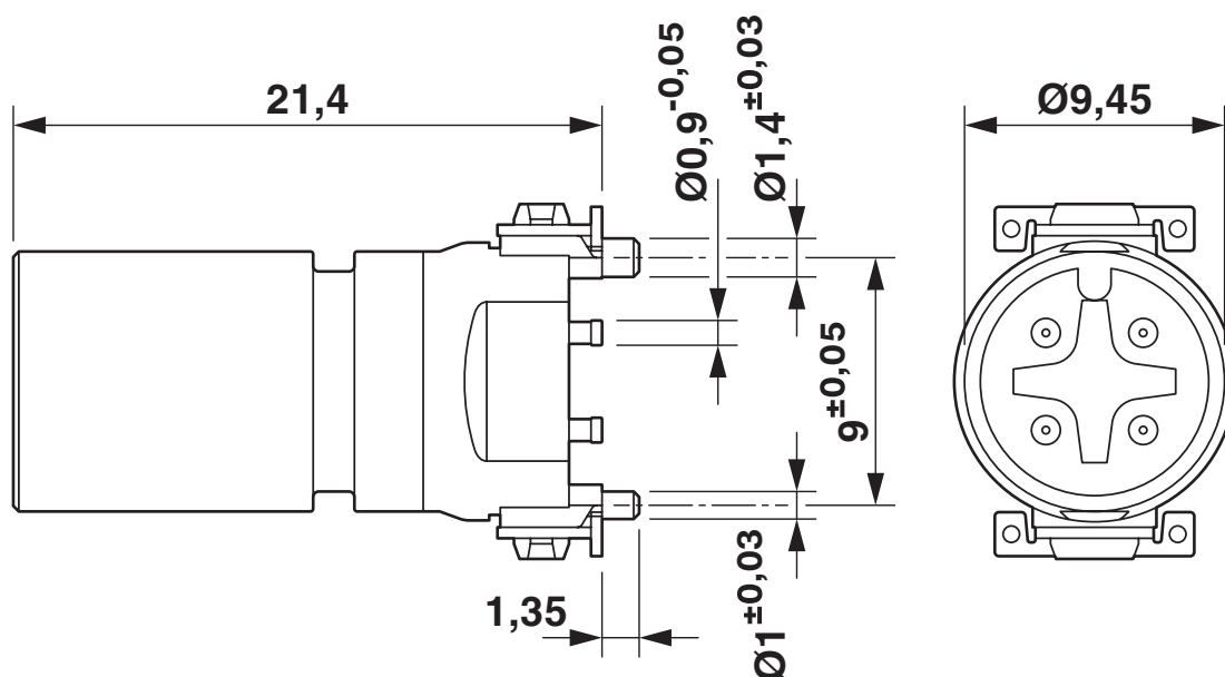
M12 male connector contact carrier
