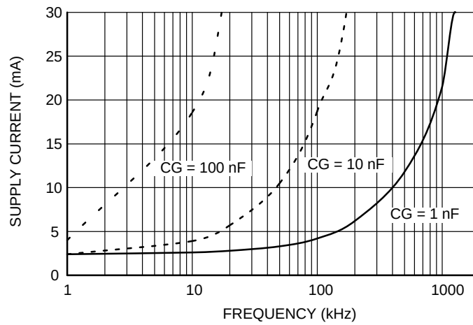
Figure 18. Supply Current vs. Switching Frequency ( V_{CC} = 15\text{ V} , 25^{\circ}\text{C} )
