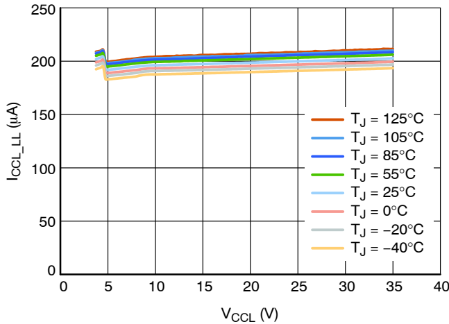
Figure 10. VCCL Current Consumption in Disable by LLD Function, V CS = 4 V, t > t LLD
