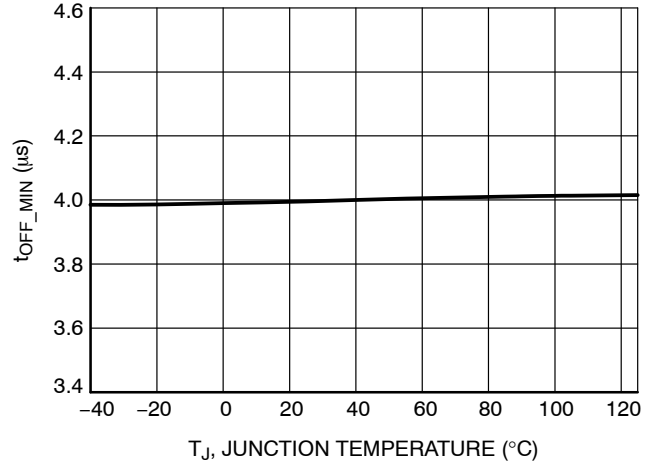
Figure 39. Minimum Off-time t_{OFF\_MIN} = 4 \mu\text{s}
