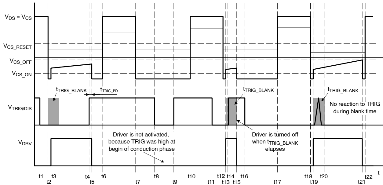
Figure 70. Trigger Input Functionality Waveforms Using the Trigger to Turn-off and Block the DRV Signal
