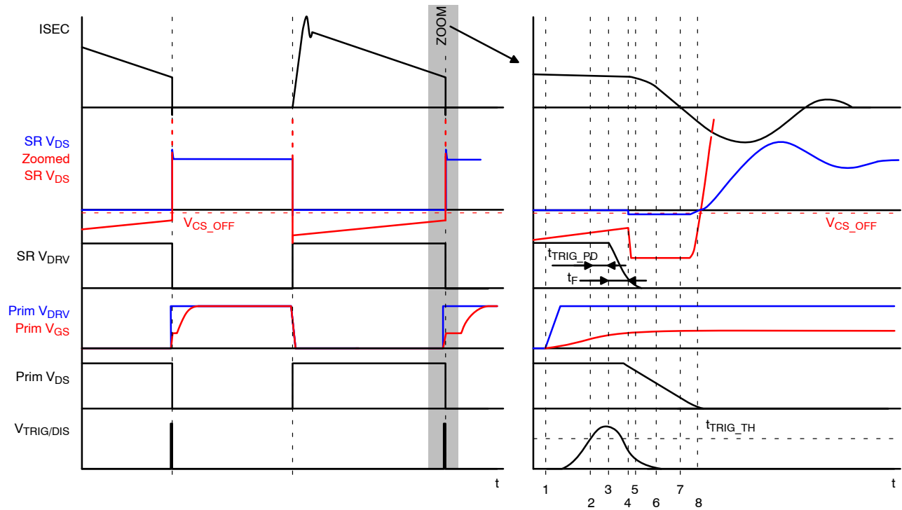
Figure 73. CCM Operation with Triggering from Primary Side
