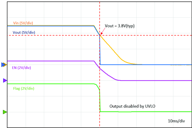
Figure 7. UVLO
