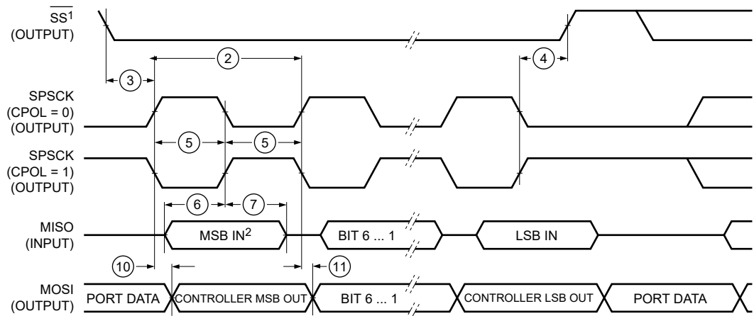
Figure 18. LPSPI Controller Mode Timing (CPHA=1)
