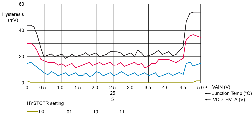
Figure 12. Typical Hysteresis vs VAIN (VDD_HV_A = 5 V, Low Speed Mode).png
