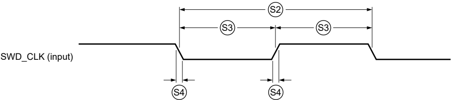
Figure 22. SWD Input Clock Timing
