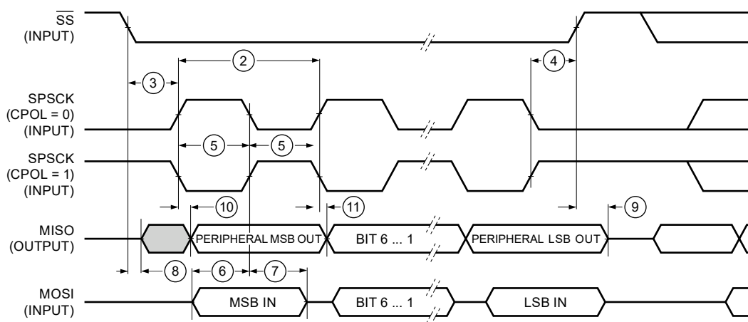
Figure 15. LPSPI Peripheral Mode Timing (CPHA=1)
