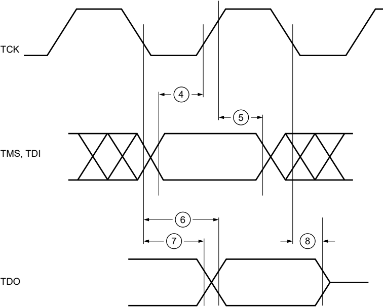
Figure 20. JTAG Test Access Port Timing
