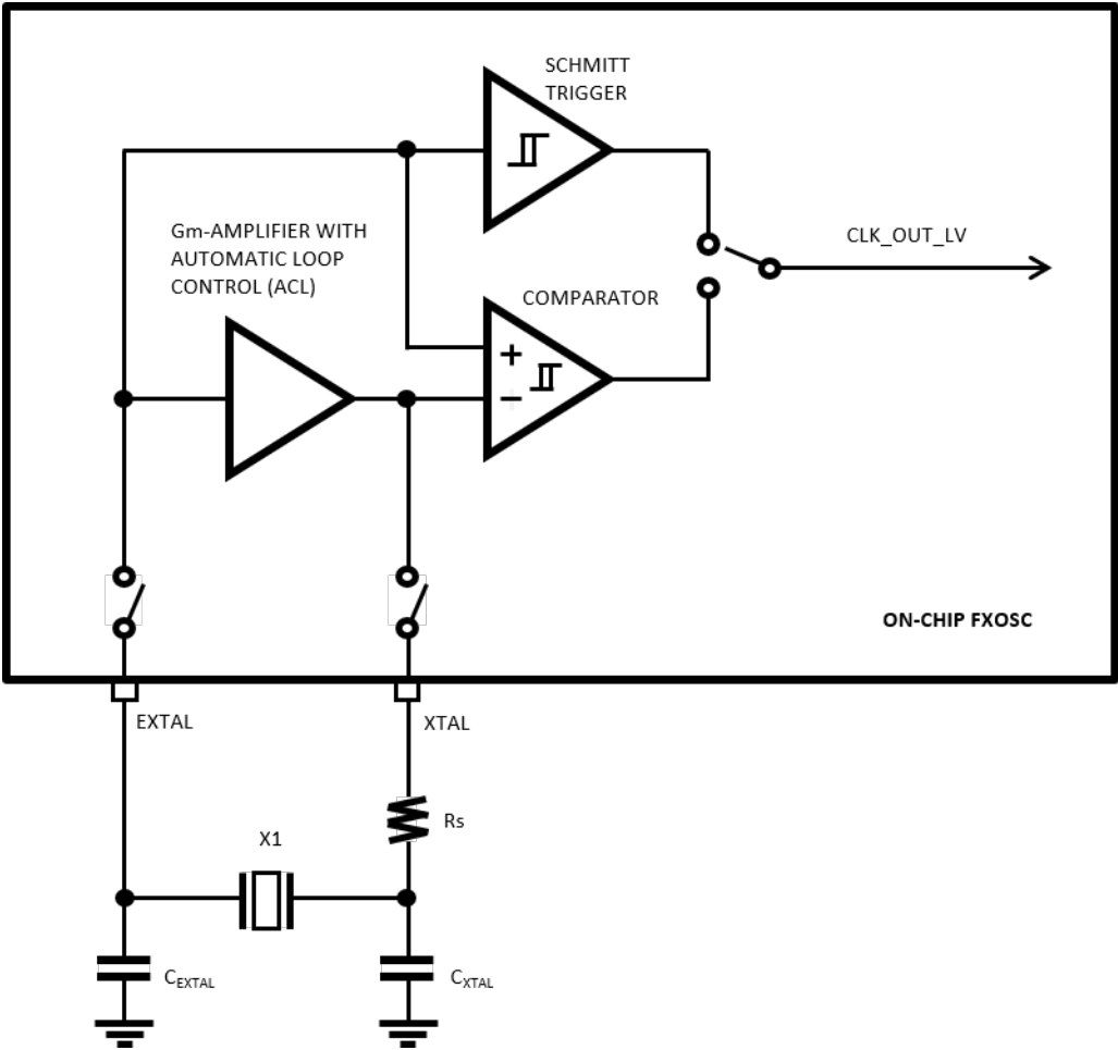
Figure 14. Block diagram
