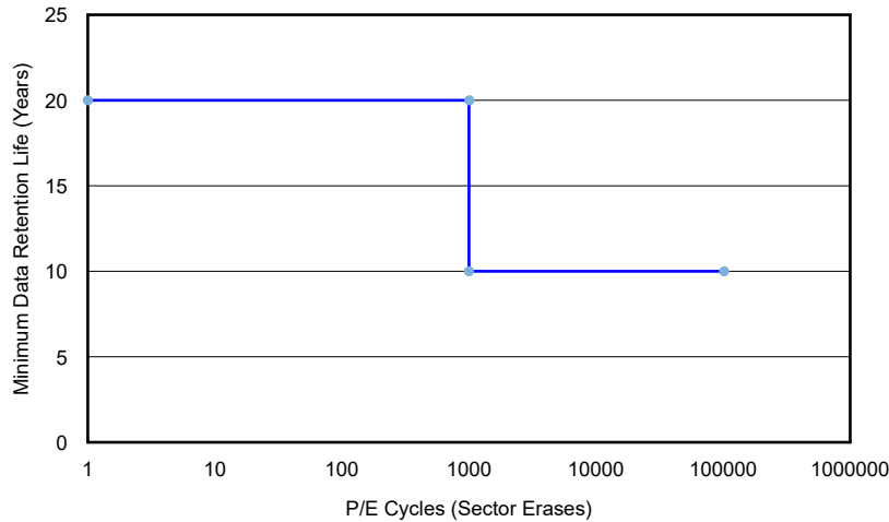
Figure 7. Data retention vs program/erase cycles
