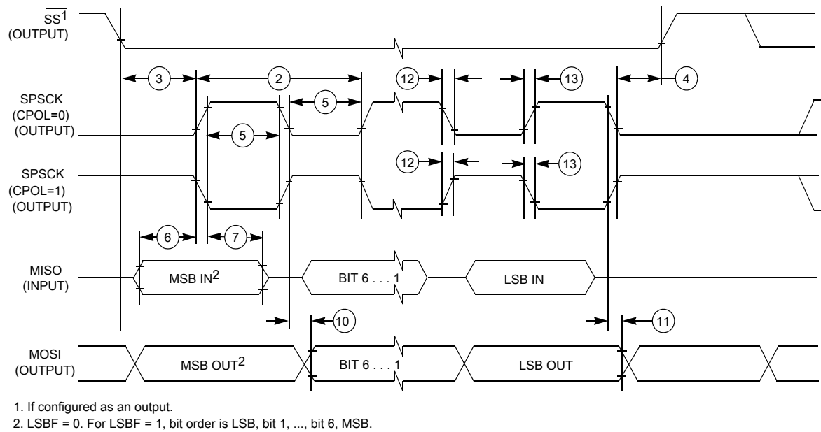
Figure 31. LPSPi master mode timing (CPHA = 0)
