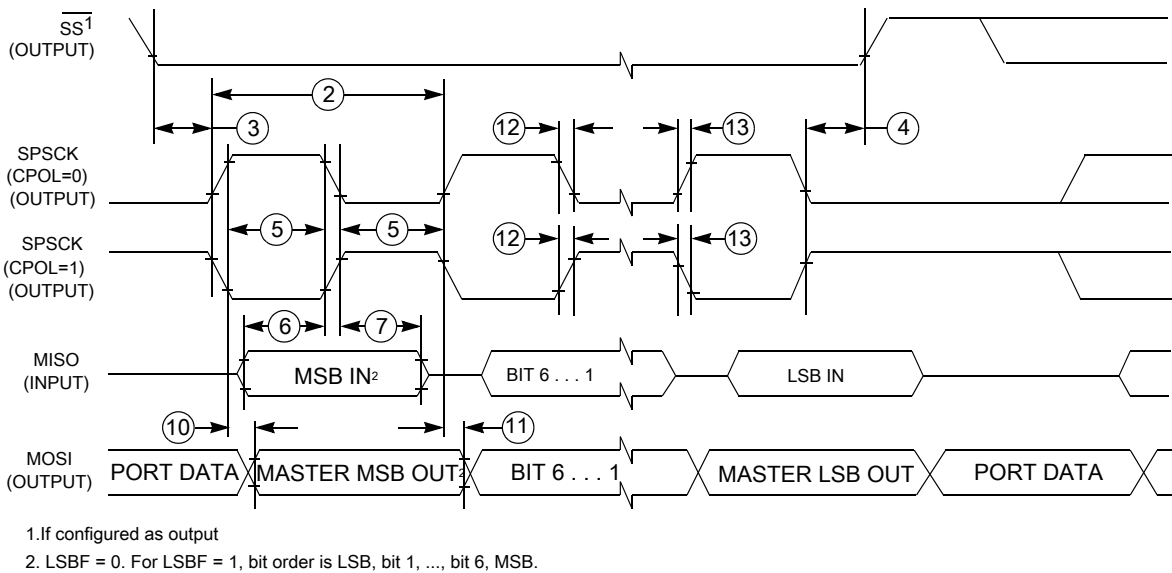
Figure 32. LPSPi master mode timing (CPHA = 1)
