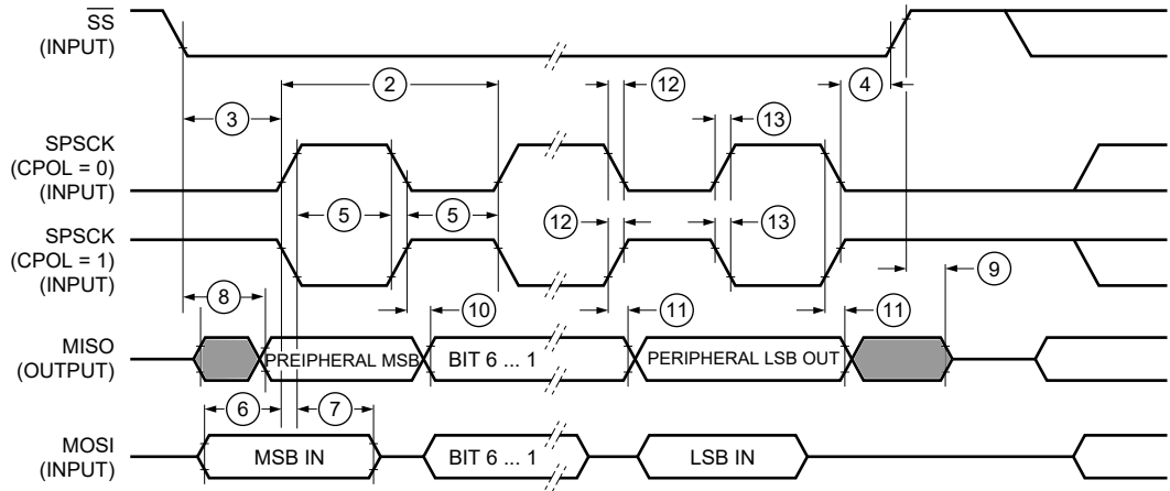
Figure 16. LPSPI Peripheral Mode Timing (CPHA=0)
