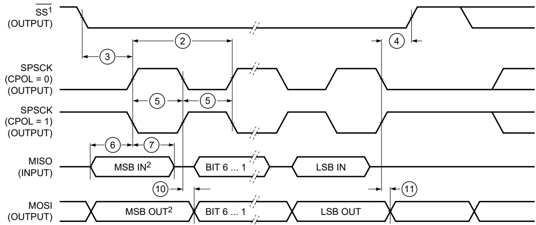
Figure 17. LPSPI Controller Mode Timing (CPHA=0)
