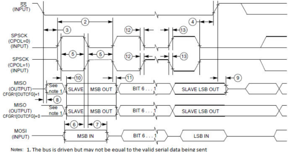
Figure 34. LPSPi slave mode timing (CPHA = 1)
