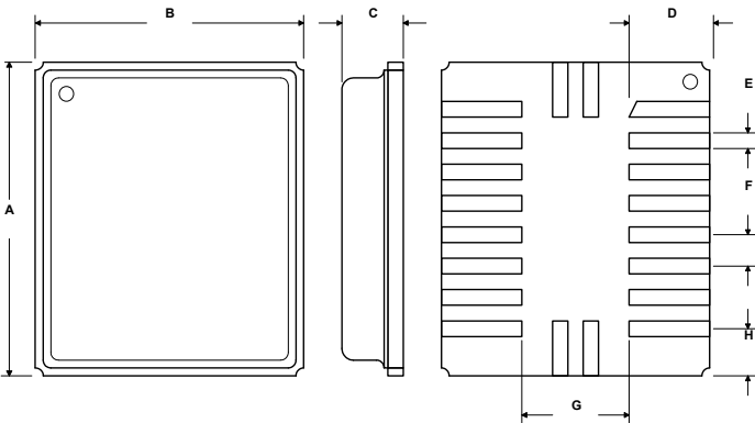
SM-20L Package Drawing
