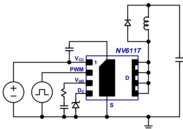
Fig. 1. Inductive switching circuit
