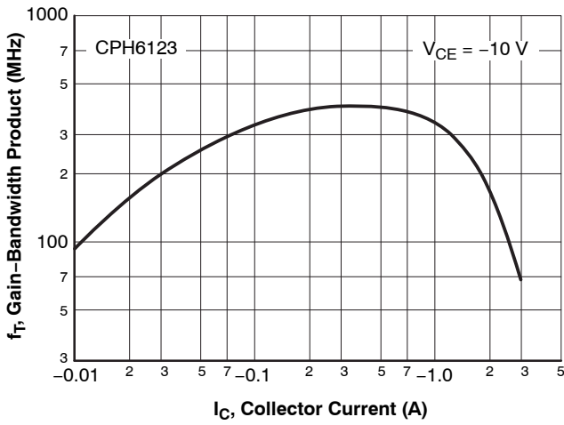
Figure 8. f_T - I_C
